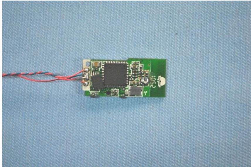
Main & RF board solder side
