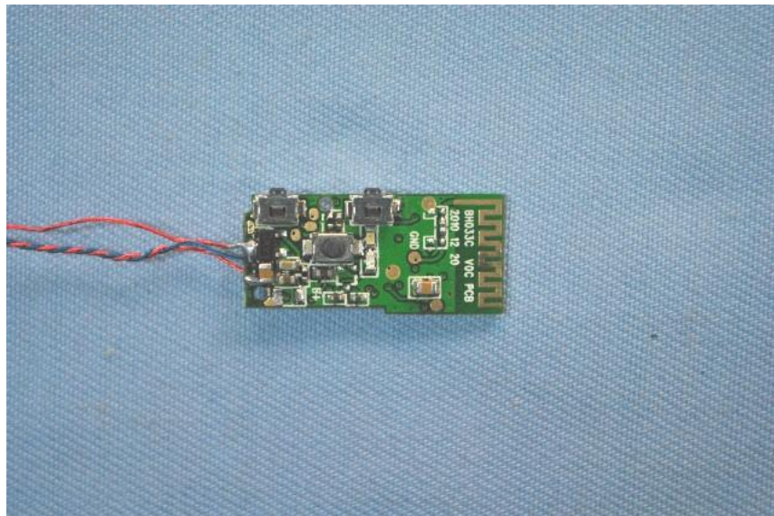
Main & RF board component side
