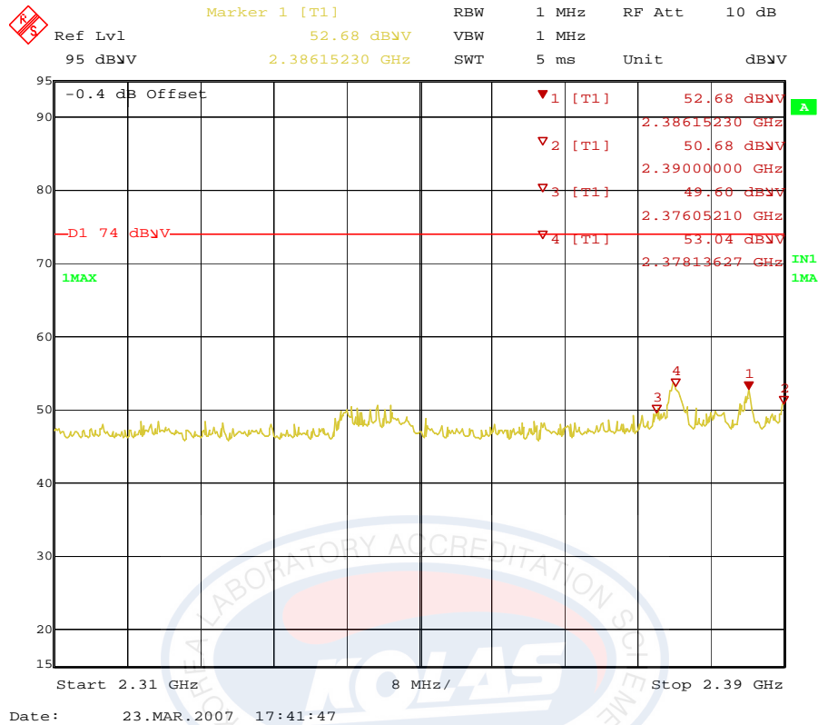
Figure 8. Plot of the Band Edge (Radiated); Internal Antenna
