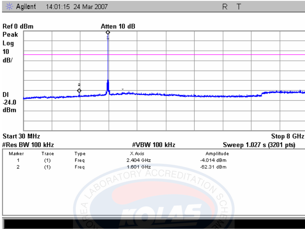
Figure 9. Plot of the RF antenna port emissions (Conducted)
