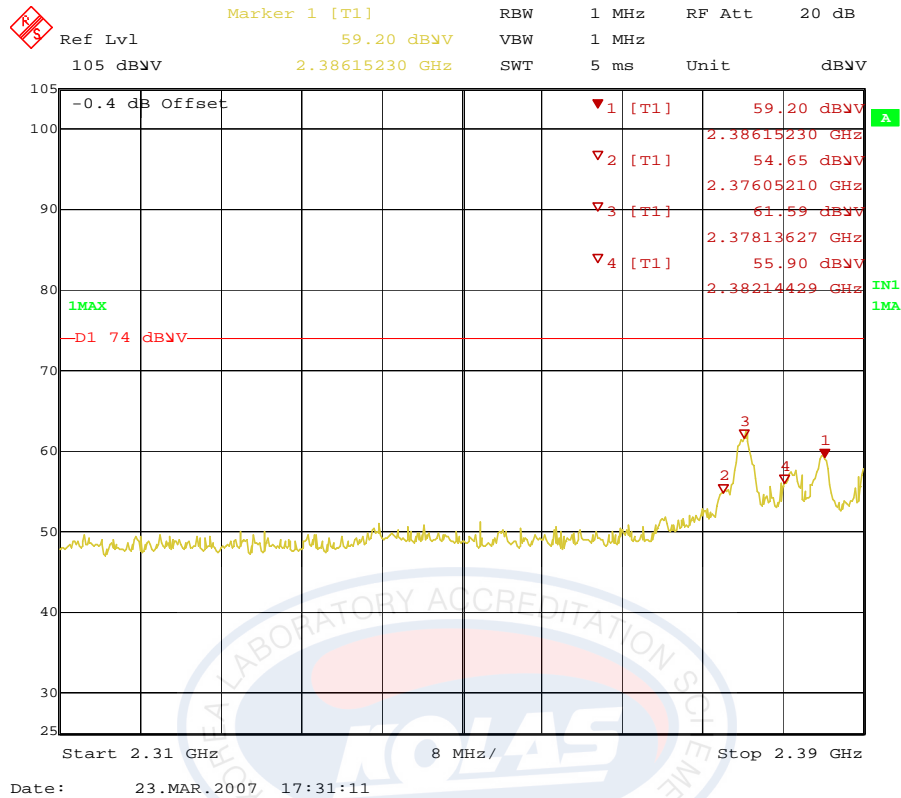
Figure 7. Plot of the Band Edge (Radiated); External Antenna
