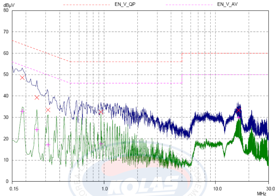
Figure 11. Plot of the Conducted Emissions
