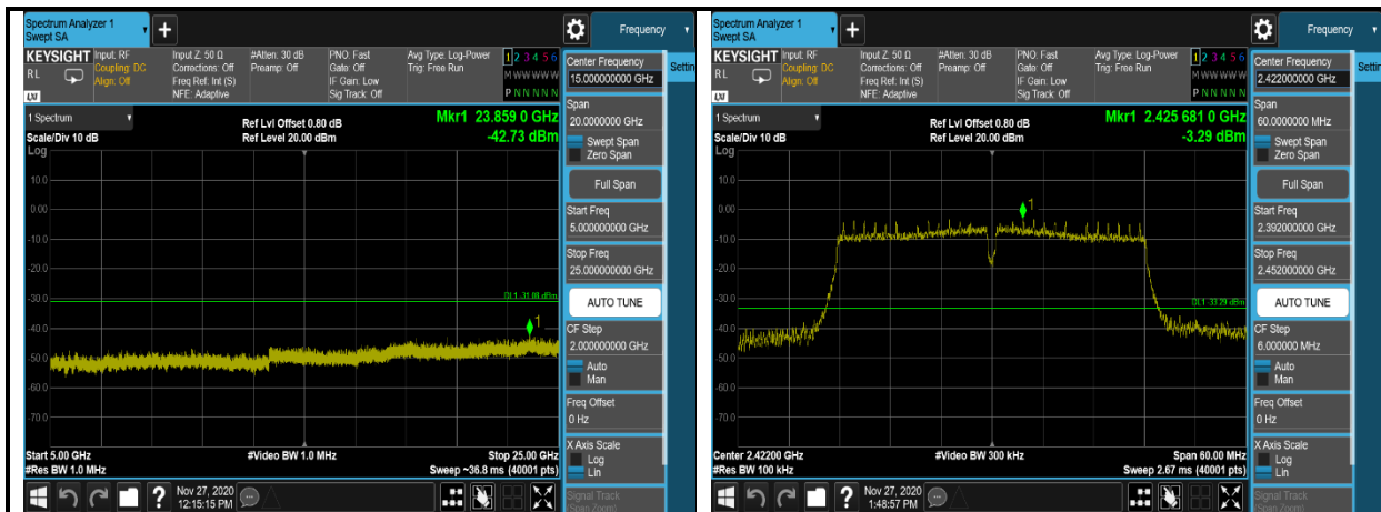
802.11n(HT40),2422MHz,Ant1,Plot 2,Band Edge
