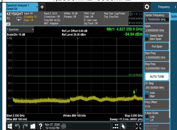
802.11n(HT40),2422MHz,Ant1,Plot 1,Reference Level
