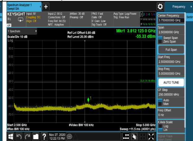
802.11n(HT40),2437MHz,Ant1,Plot 1,Reference Level
