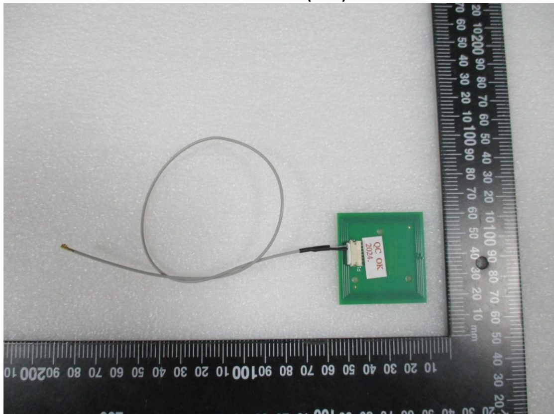
RFID Antenna (New)
