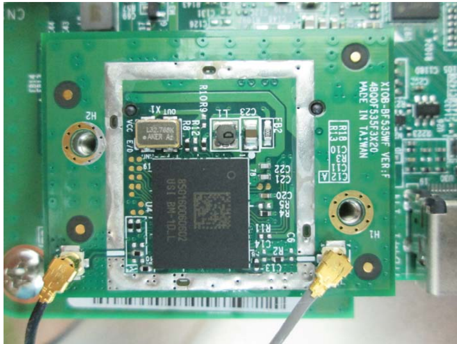
WiFi Combo Antenna connection
