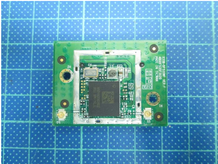
WiFi Combo module
