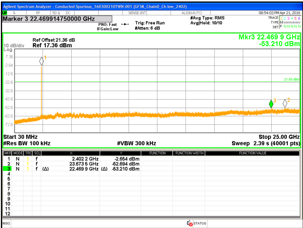
Chain0 : Conducted Spurious @ Ch Low
