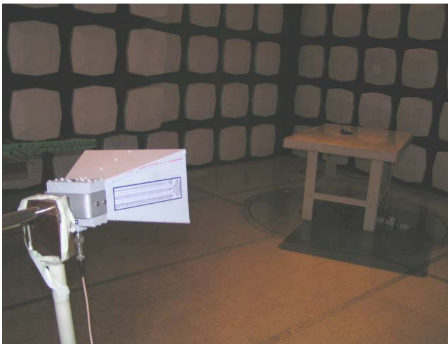
Radiated emission test setup - high frequency
