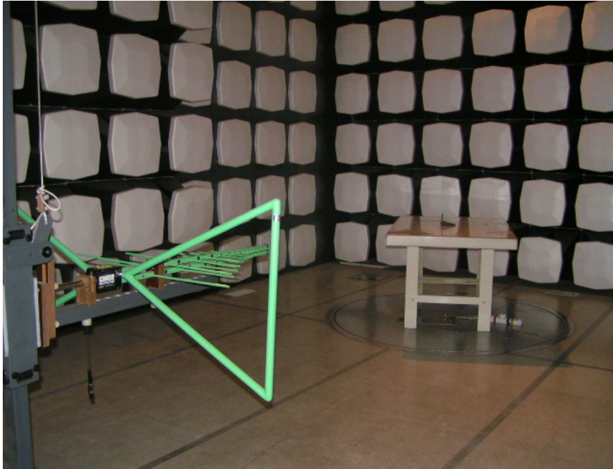
Radiated emission test setup - low frequency
