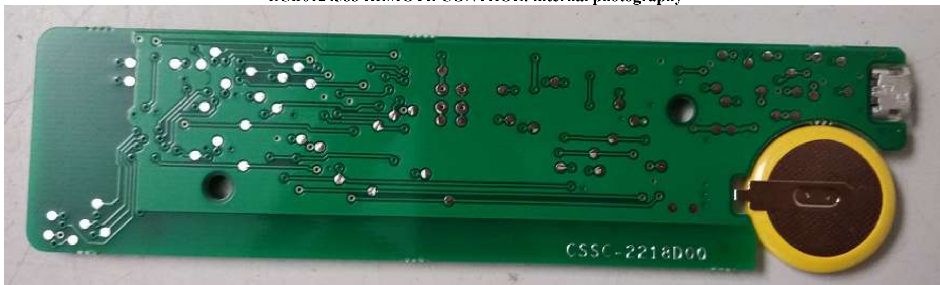
ECB0124588 REMOTE CONTROL: internal photography
