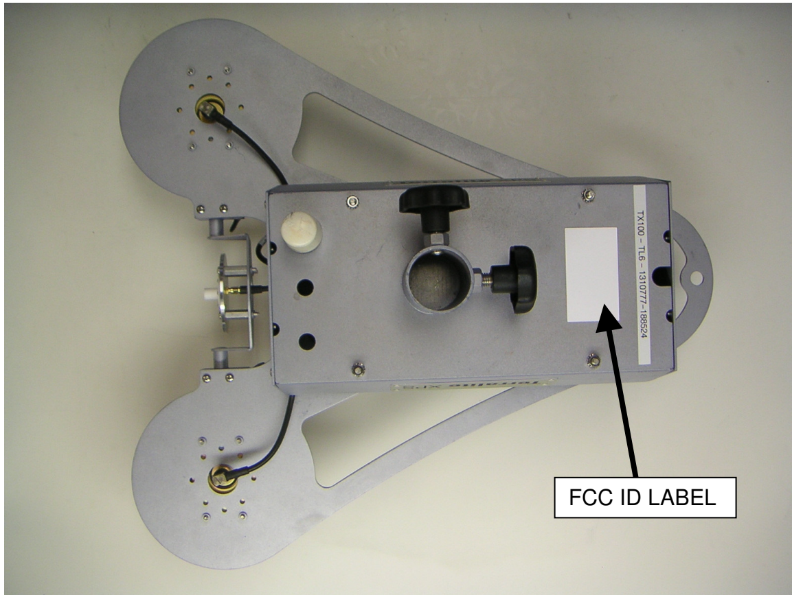
Figure 1: FCC ID Label Location. In use, the device is mounted on a 6 to 8 foot tall post, therefore an underside location was deemed easily accessible and readable.
