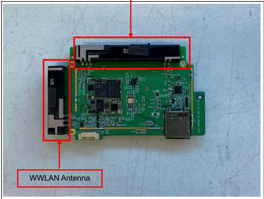
WWLAN + GPS Antenna (Only Rx)
