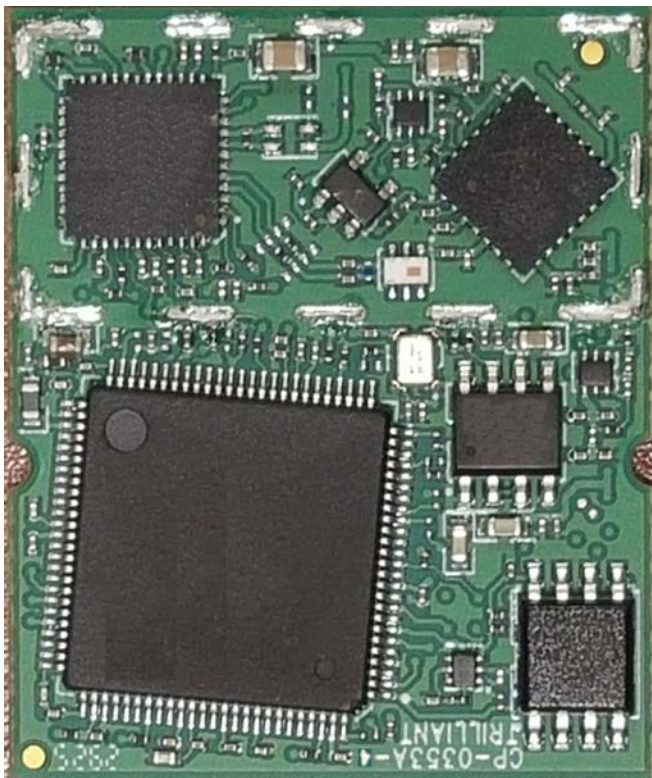
No shield: CL-R0353A-6.2 (left), CL-R0368A-1.1 &amp; CL-R0368B-1.0 (right)
