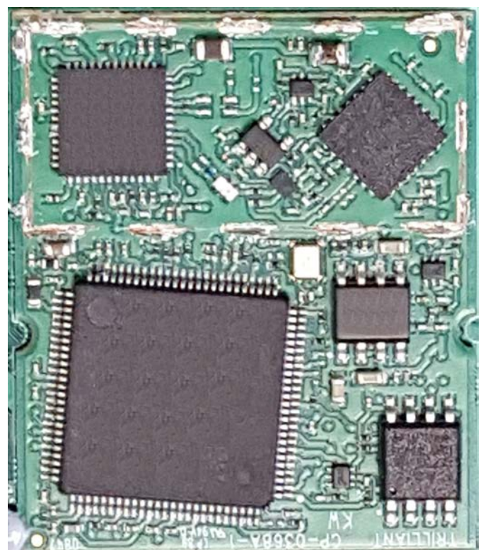
No shield: CL-R0353A-6.2 (left), CL-R0368A-1.1 &amp; CL-R0368B-1.0 (right)
