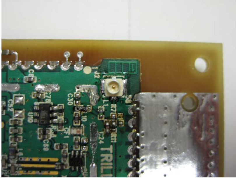
Close Up of Antenna Connection on Board (Model EM-0069B)
