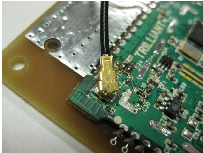
Close Up of U.FL to SMA Cable Connected to Module (Model EM-0069B)
