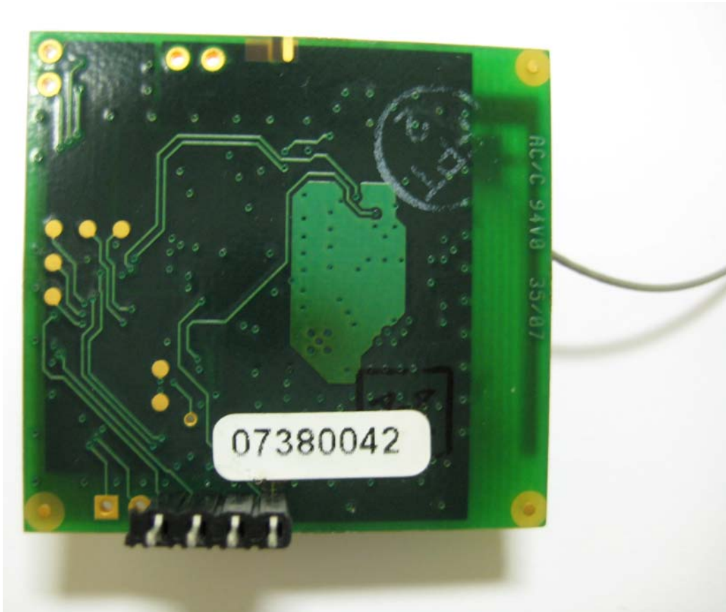
Back Side of Board – View 1
