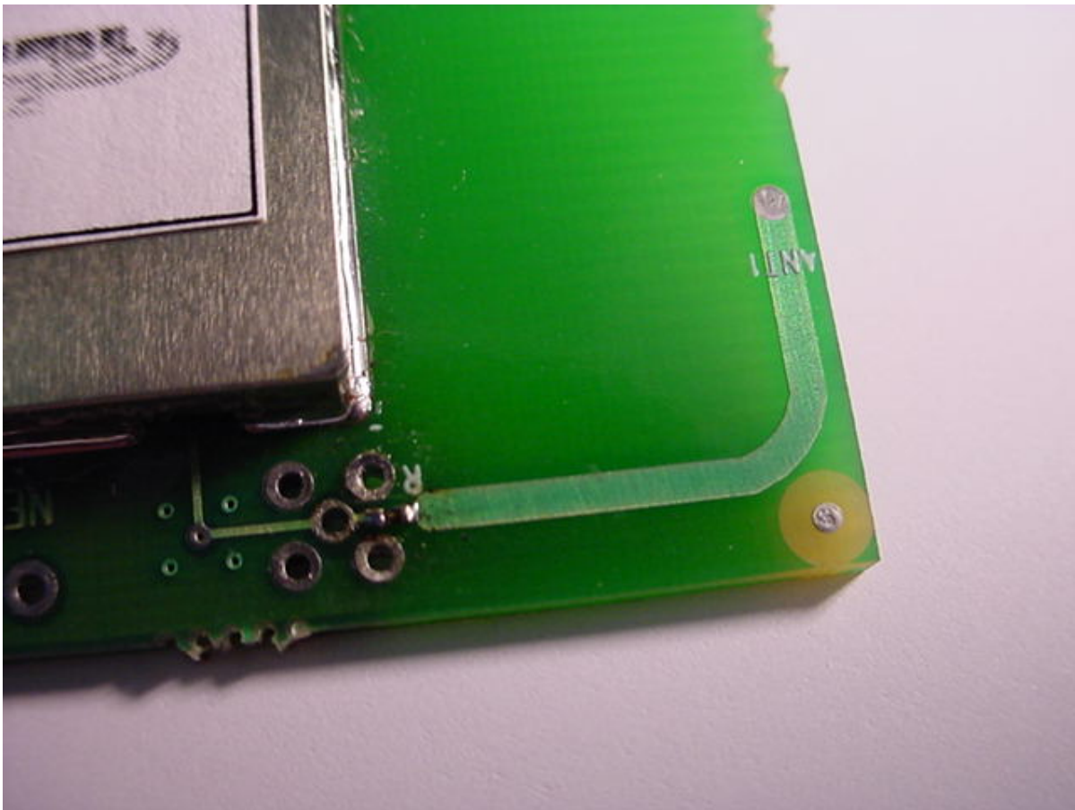
Photo Three – External View of Antenna
