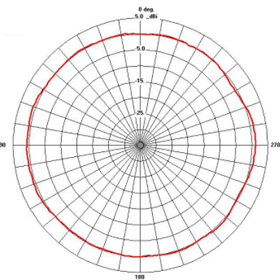
Azimuth WCR2400MMCX
