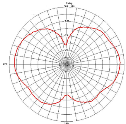
Elevation WCR2400MMCX
