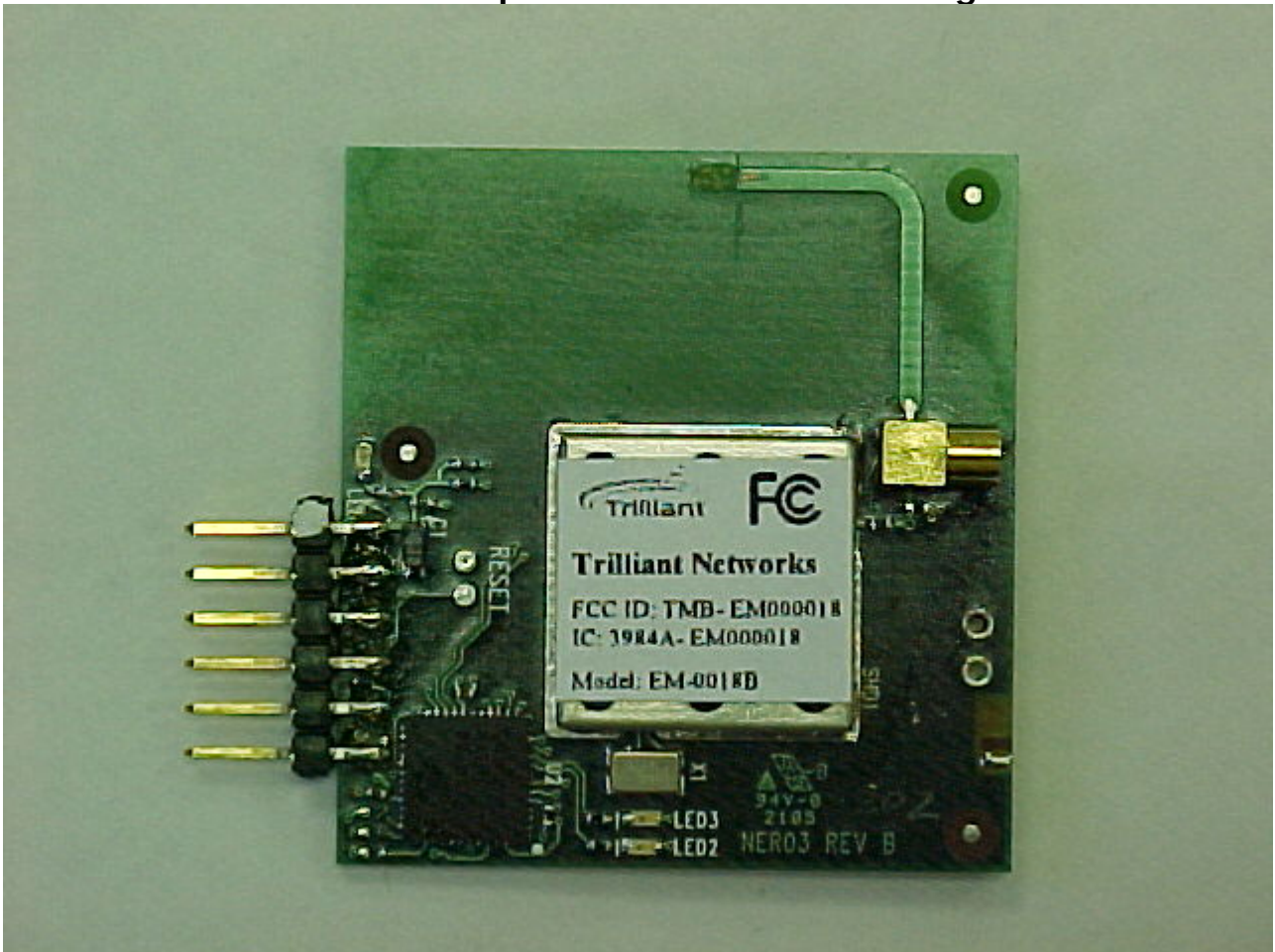
Photo Five – External RF Module-Component Side with Shielding
