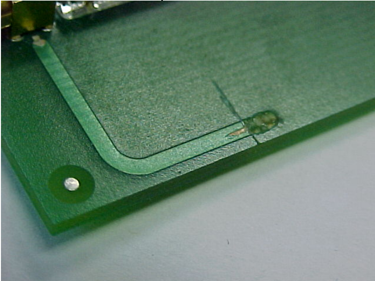
Photo Four – External Close-up of PCB Antenna
