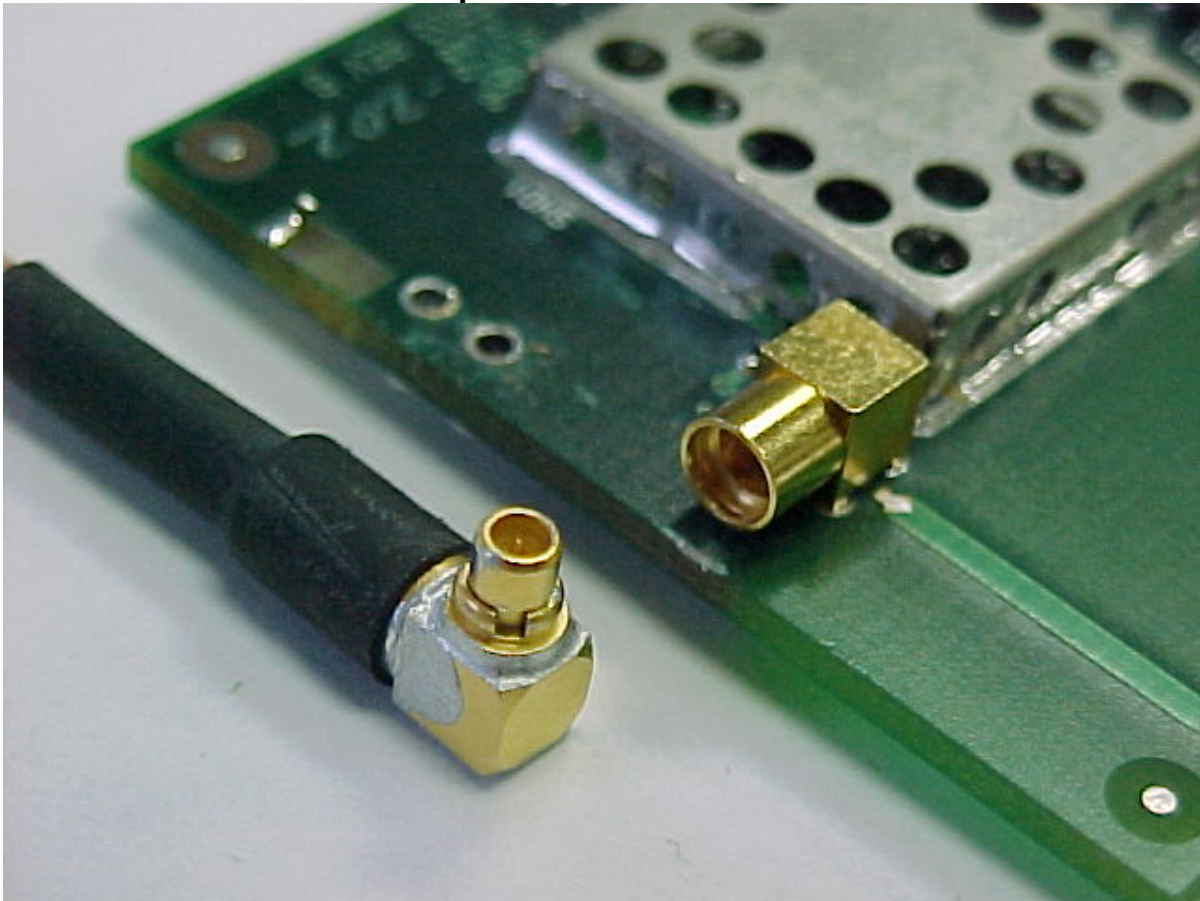
Photo Three – External Close-up of Antenna Connector
