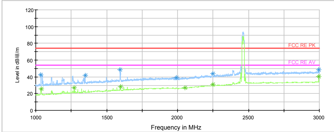
RE 1G-3GHz PK+AV
