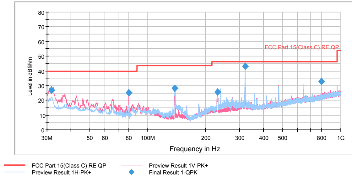
RE 30M-1GHz QP
