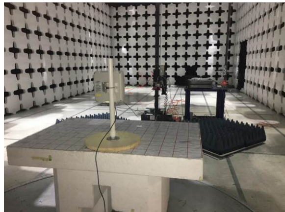
Radiated Emissions Above 1GHz - Rear View
