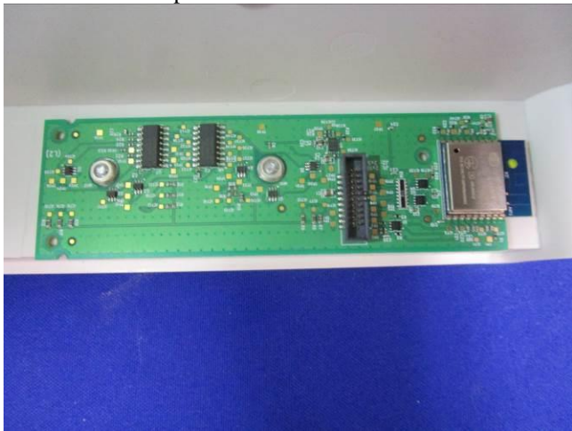
2.4Ghz Control Board View
