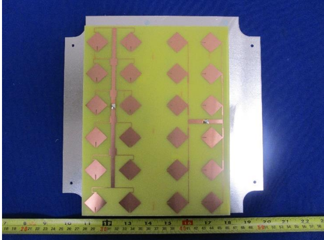
5Ghz Antenna Top View
