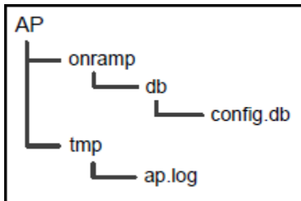
Figure 33. File structure
