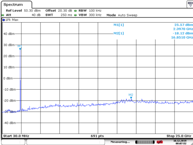
Figure 8.7-1: Conducted spurious (out-of-band) emissions, low channel
