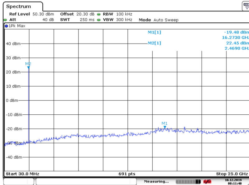
Figure 8.7-3: Conducted spurious (out-of-band) emissions, high channel
