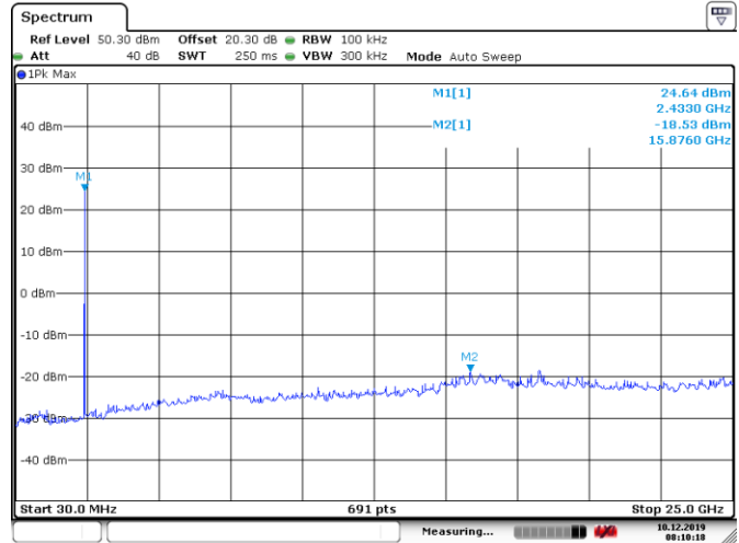
Figure 8.7-2: Conducted spurious (out-of-band) emissions, mid channel
