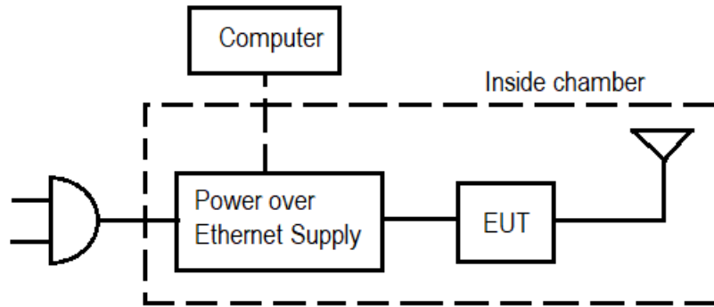
Figure 3.6-1: Setup diagram
