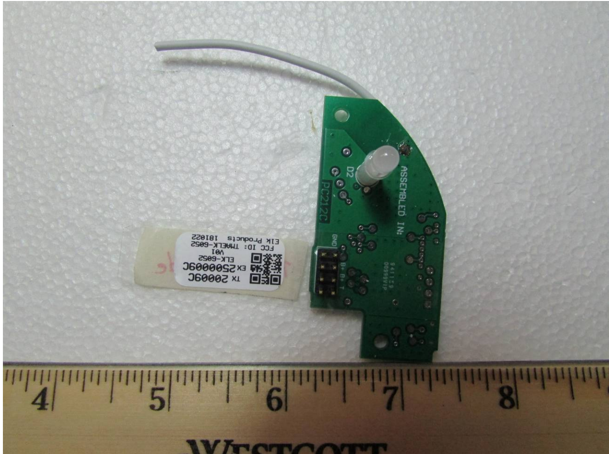
Figure 4: PCB bottom
