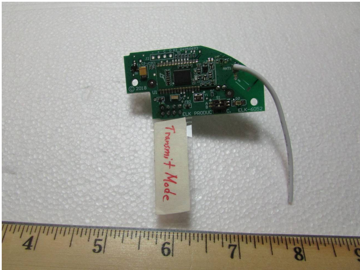
Figure 5: PCB Top
