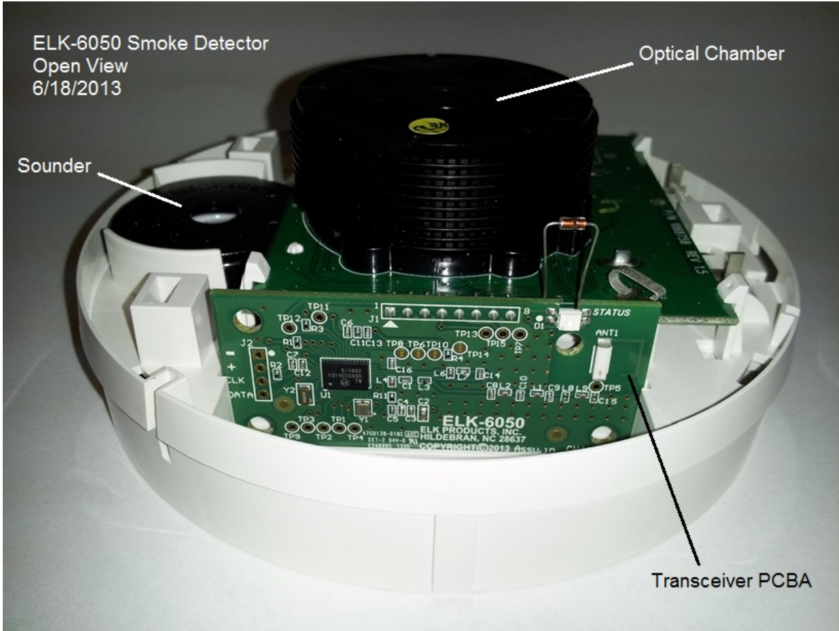
ELK-6050 With Cover Removed:
