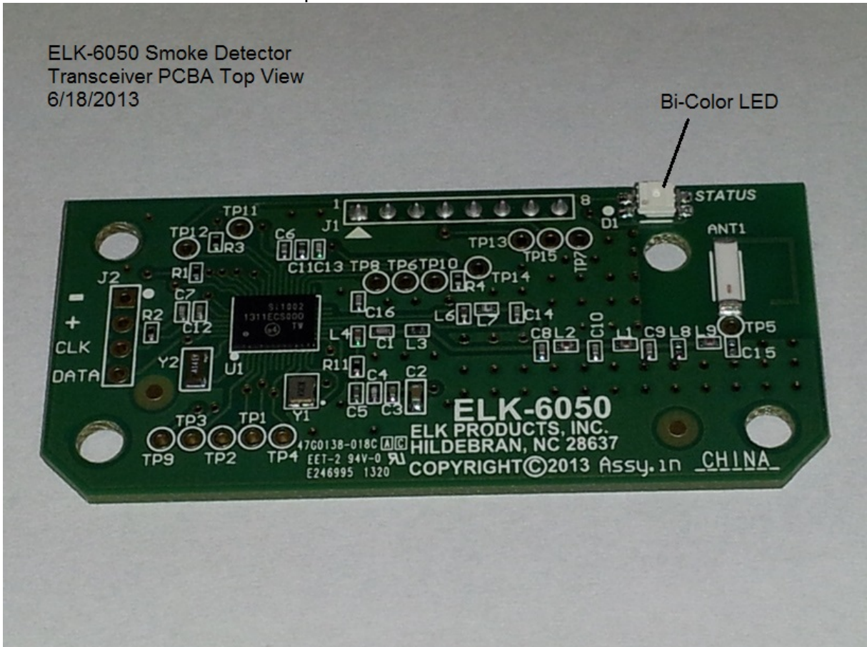
ELK-6050 Transceiver PCBA Top:
