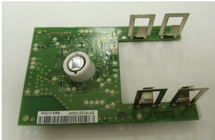
ELK-6030 PCB Top View (Top faces away from the wall):
