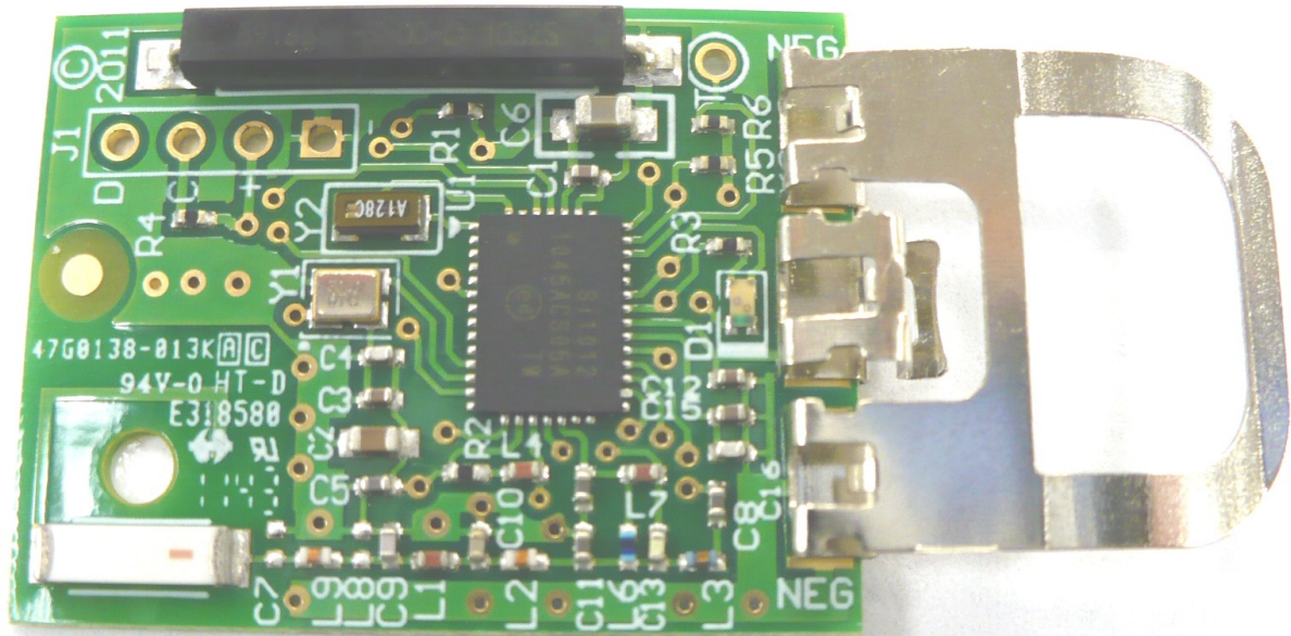
ELK-6021 PCB Front View
