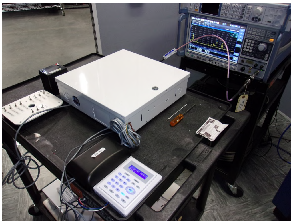
Photo 1.1-1 – Conducted Test Setup
