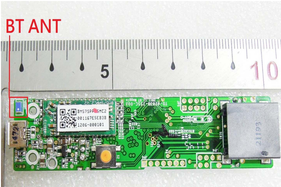
Antenna Location
