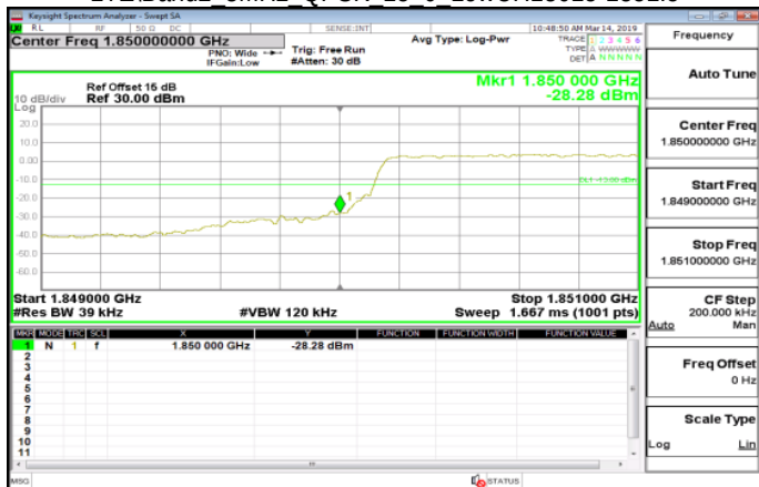
LTE\Band2 3MHz QPSK 15 0 LowCH18615-1851.5
