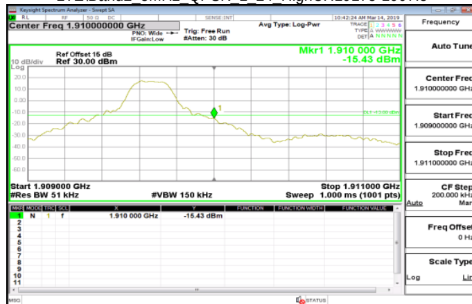
LTE\Band2 5MHz QPSK 1 24 HighCH19175-1907.5
