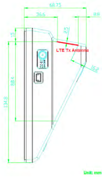
Fig.12 Antenna location of EUT
