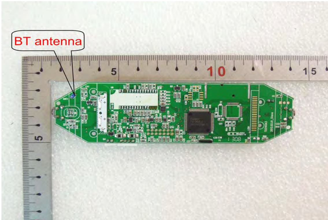
BT Antenna-2
