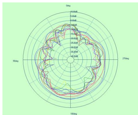
Theta90
