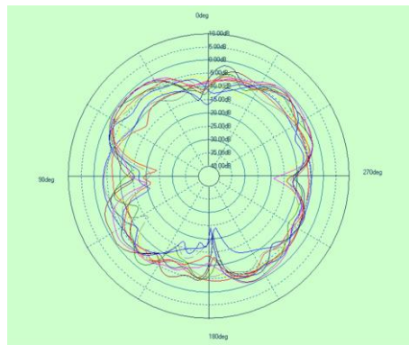
Phi 90
