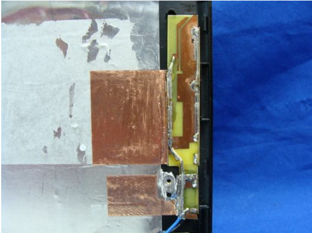
(18) EUT Photo [YAGEO, CAN43139LWPE00402 (R) / CAN43139LWPE00403 (L)]
