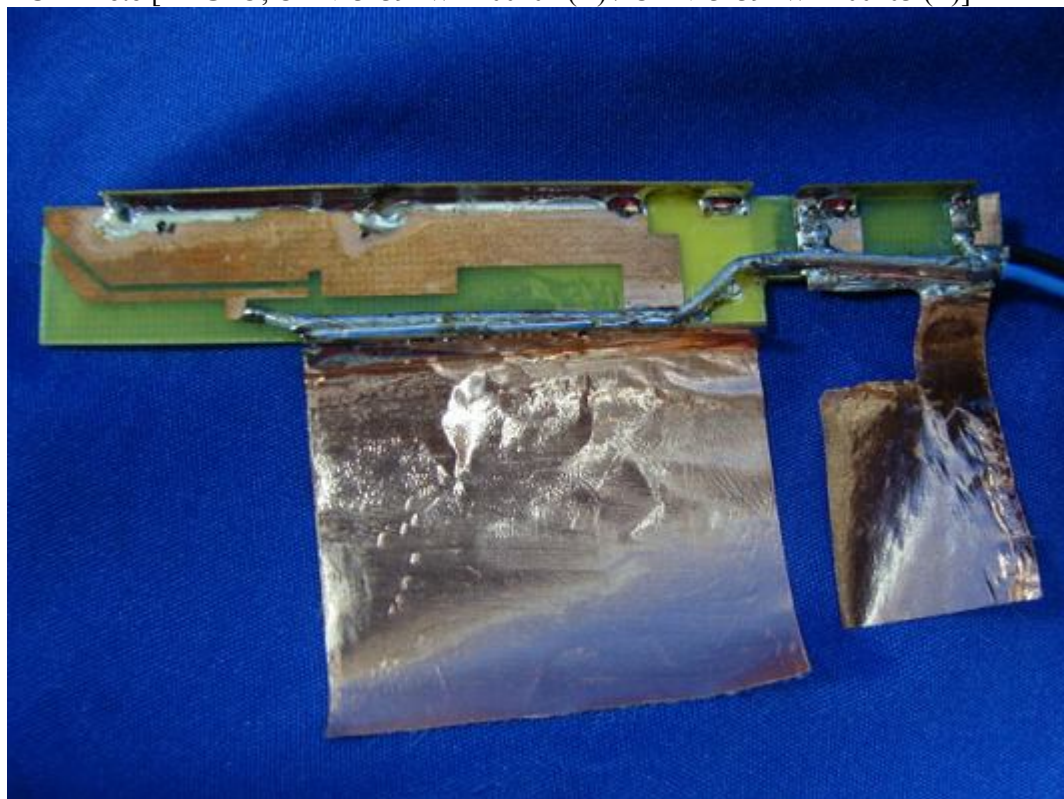
(16) EUT Photo [YAGEO, CAN43139LWPE00402 (R) / CAN43139LWPE00403 (L)]
