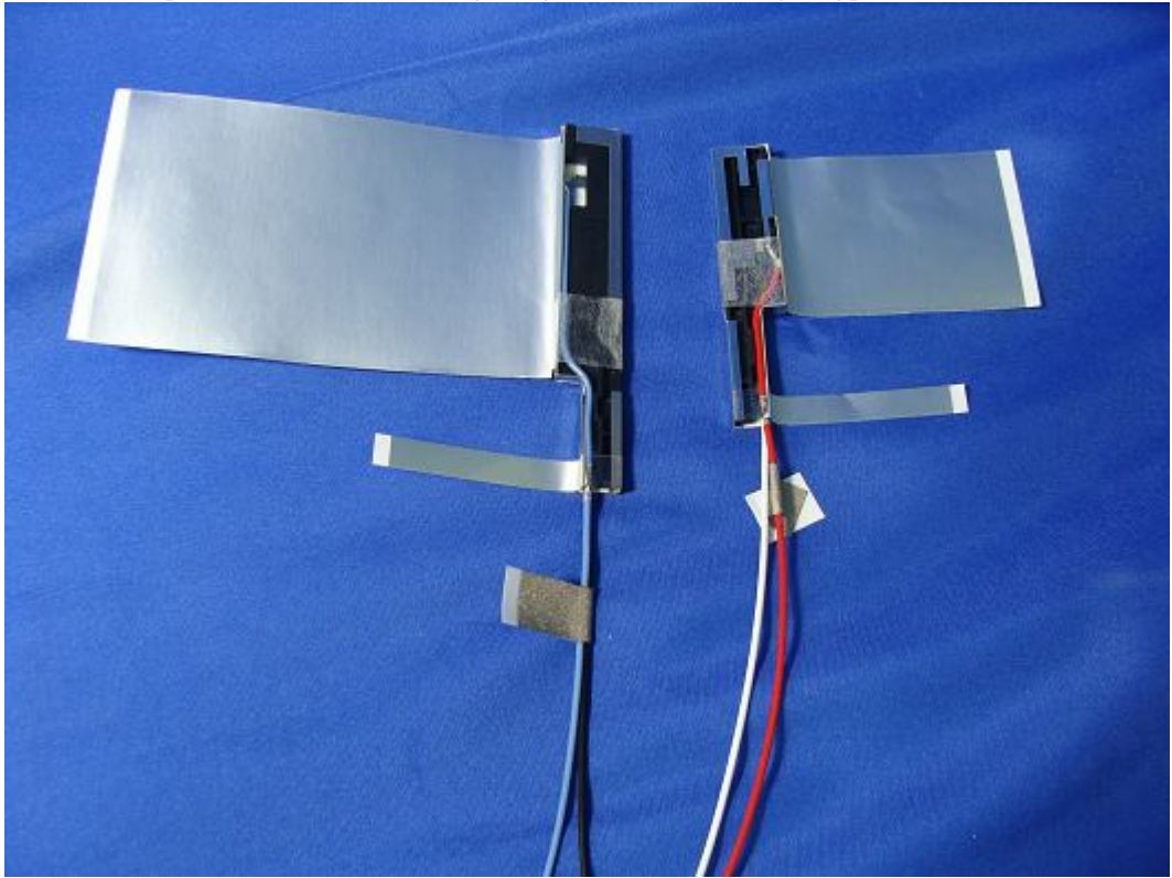
(20) EUT Photo [WNC, 81.EK815.G01 (Main), 81.EK815.G02 (Aux)]
