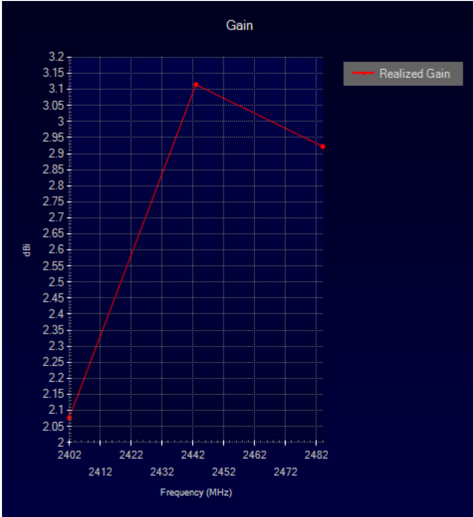
Figure 1 : Gain Chart
