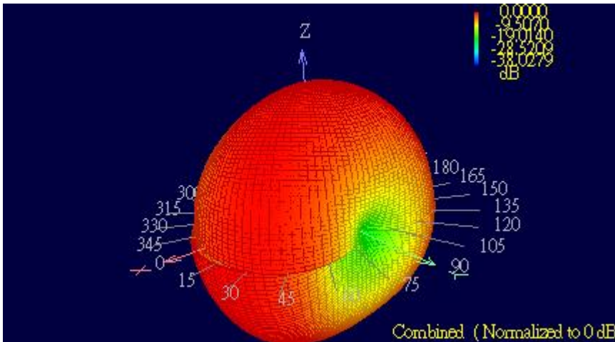
Figure 2 : 3D Far-Field Combined
