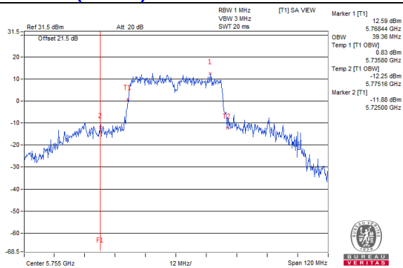
802.11ac(VHT40) / CH151
