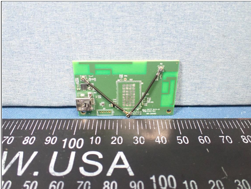
PCB Antenna (Brand: lynwave / Model: 5-PP005049)
