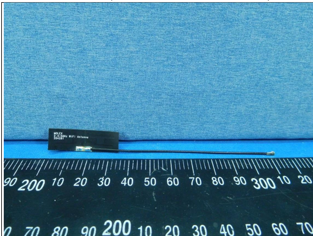
PCB Antenna (Brand: Molex / Model: 2042811100)
