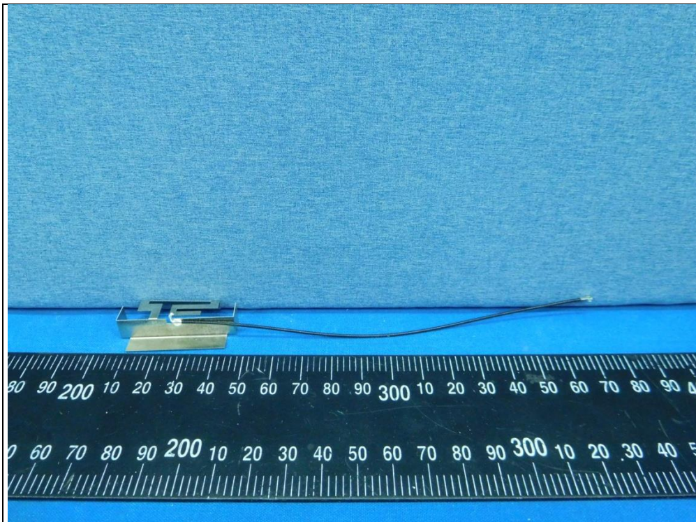
PIFA Antenna (Brand: MAG.LAYERS / Model: MSA-4008-25GC1-A2)
