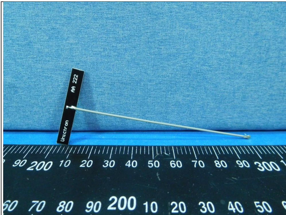
PCB Antenna (Brand: Unictron / Model: H2B1PD1A1C385L)
