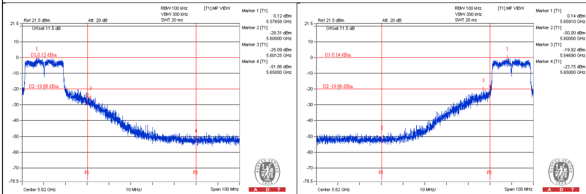
802.11ac (VHT20) MODULATION (CH 116: 5580MHz)
