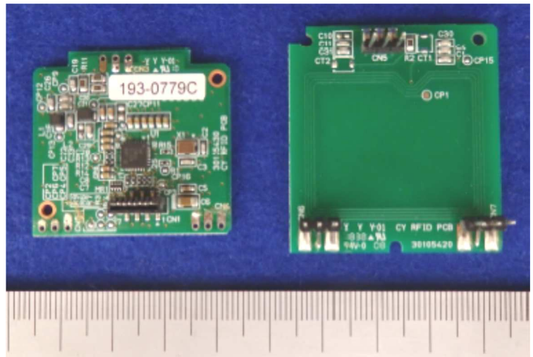
Control PCB
