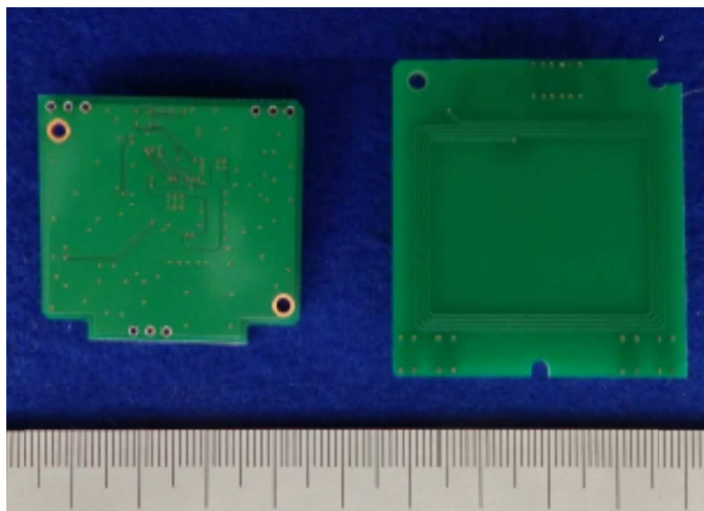
Control PCB
