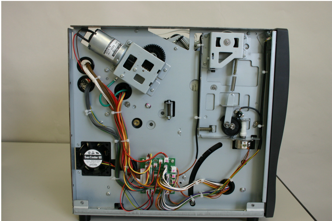
Figure 9.0-7 PHOTO PRINTER CV-01 Internal View - RIGHT
