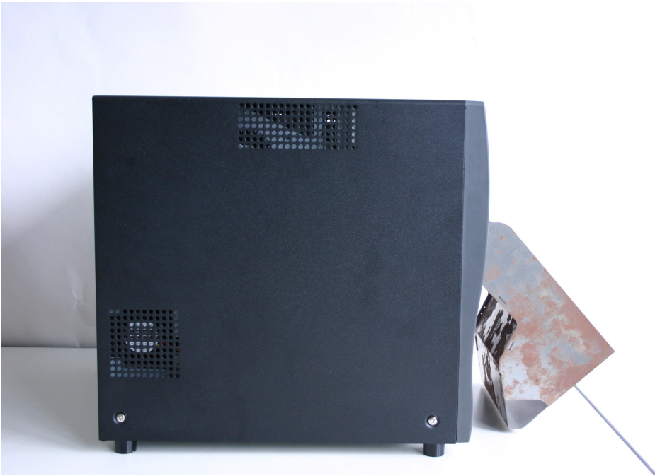
Figure 3.0-3 PHOTO PRINTER CW-01 and OPTION PAPER TRAY External View - RIGHT
