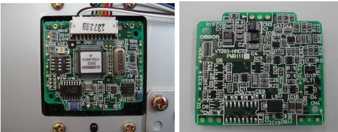
Figure 9.0-11 TOP and BOTTOM VIEW OF RFID Reader/Writer Module CONTROL BORAD
