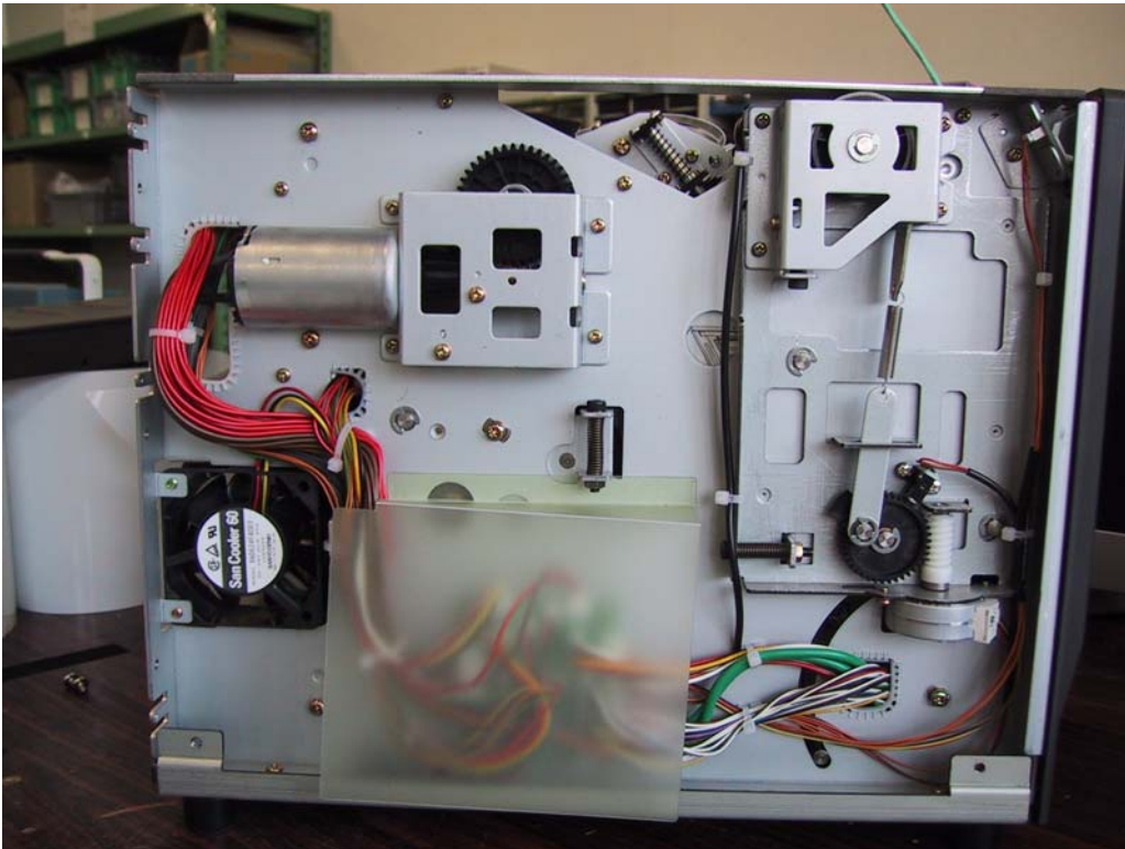
Figure 9.0-7 PHOTO PRINTER CV01-H01 Internal View - RIGHT
