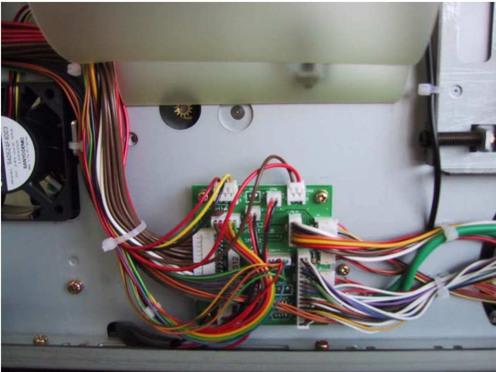
Figure 9.0-8 PHOTO PRINTER CV01-H01 Internal View - RIGHT
