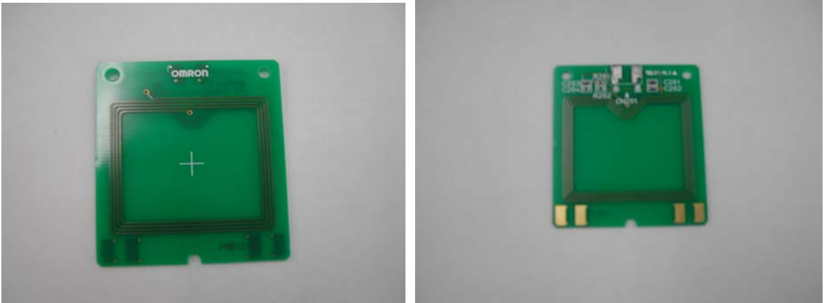
Figure 9.0-12 TOP and BOTTOM VIEW OF RFID Reader/Writer Module ANT BORAD
