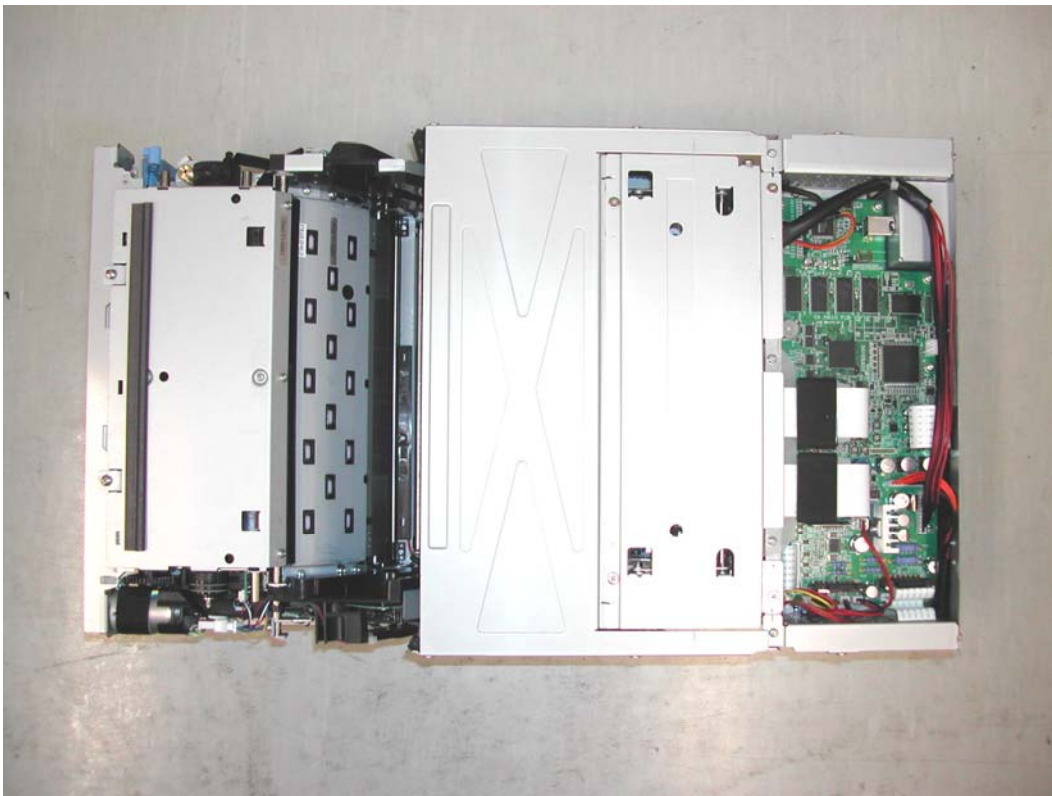
Figure 9.0-7 PHOTO PRINTER Internal View- TOP
