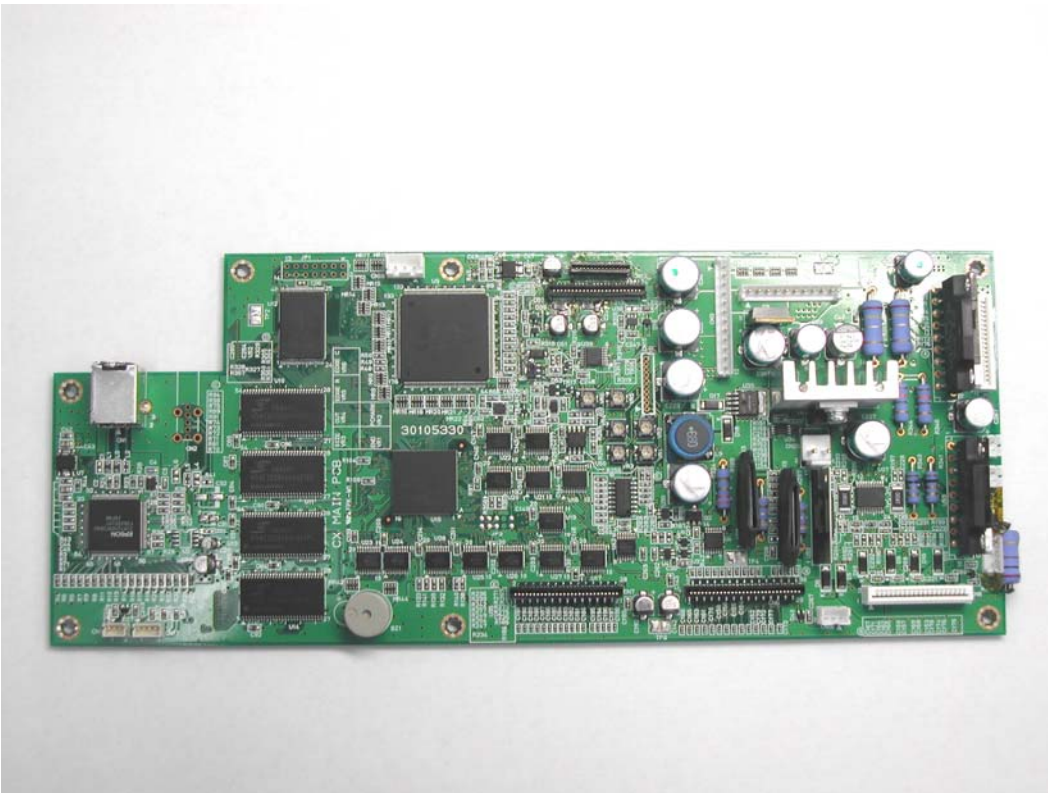
Figure 9.0-2 TOP VIEW OF MAIN BOARD
