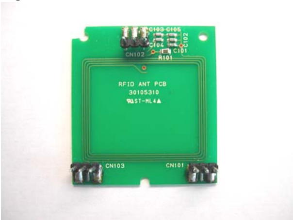
Figure 9.0-6 TOP and BOTTOM VIEW OF RFID Reader/Writer Module ANT BORAD
