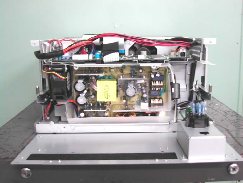
Figure 9.0-1 PHOTO PRINTER Internal View - Rear
