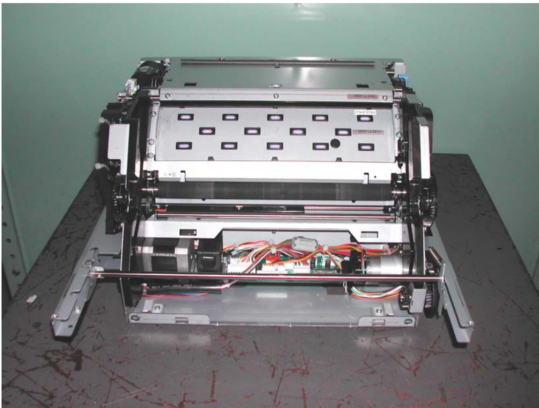
Figure 9.0-8 PHOTO PRINTER Internal View
