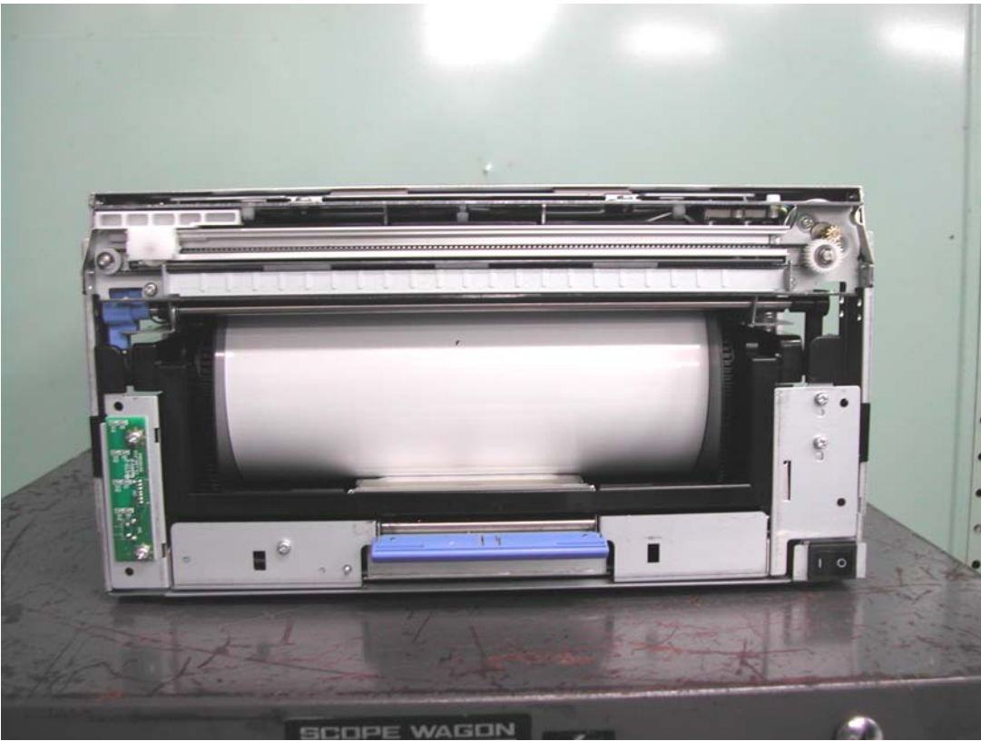
Figure 9.0-9 PHOTO PRINTER Internal View- Front
