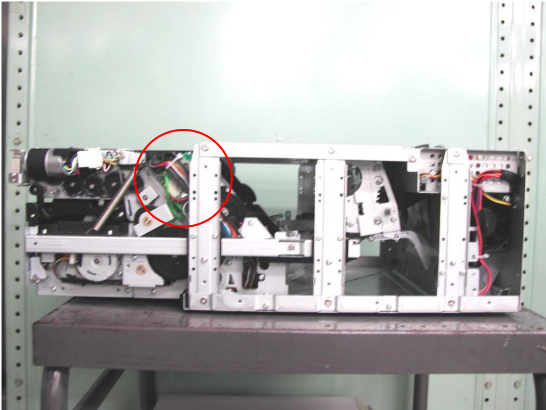
Figure 9.0-4 PHOTO PRINTER Internal View- LEFT
