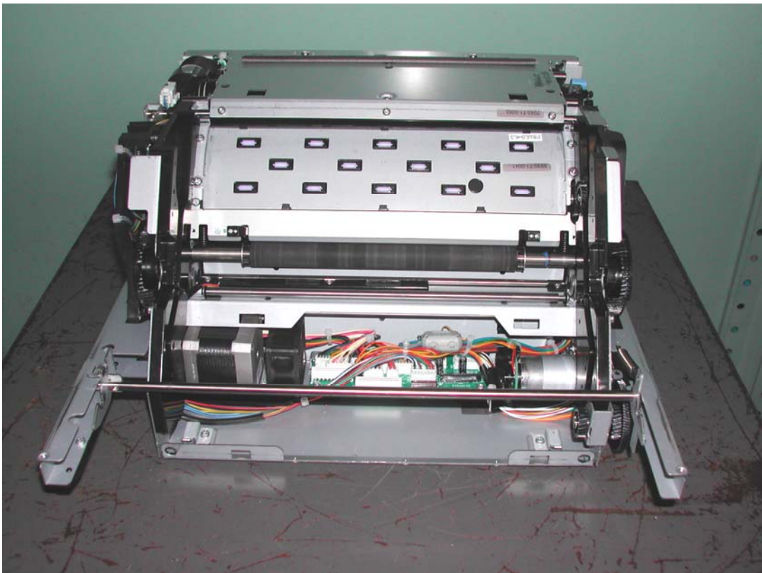
Figure 9.0-8 PHOTO PRINTER Internal View- TOP
