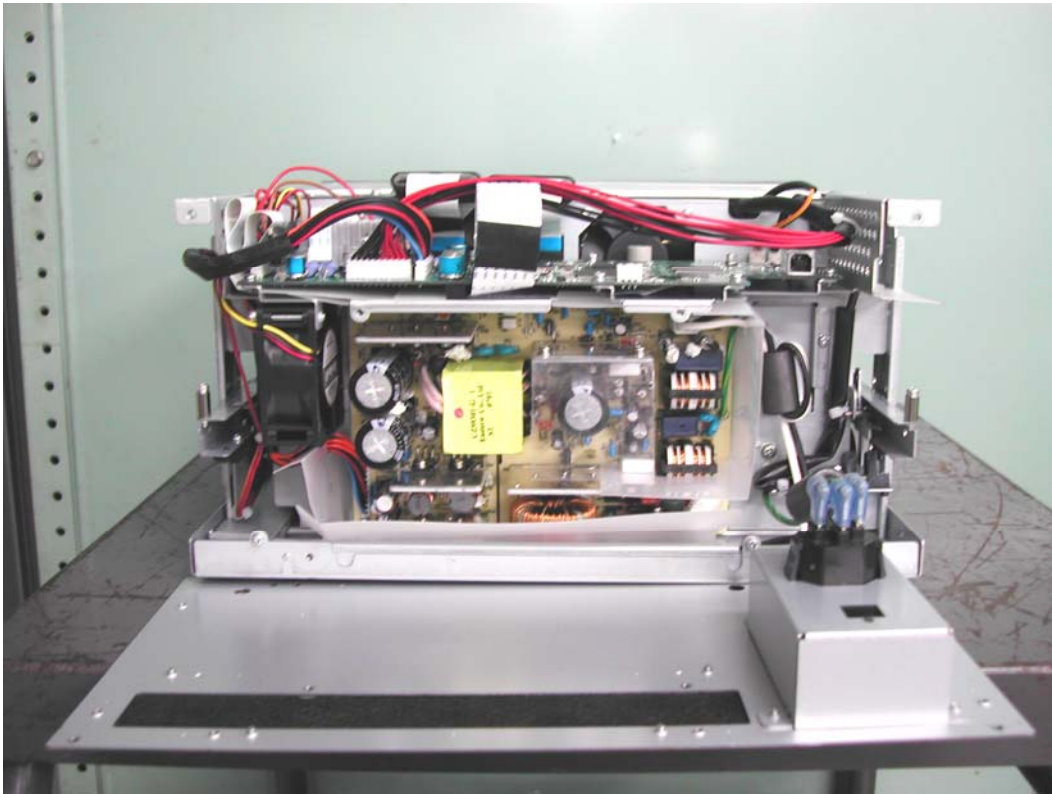
Figure 9.0-1 PHOTO PRINTER Internal View - Rear
