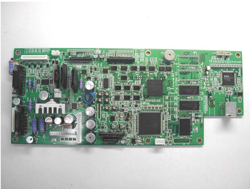
Figure 9.0-2 TOP VIEW OF MAIN BORAD
