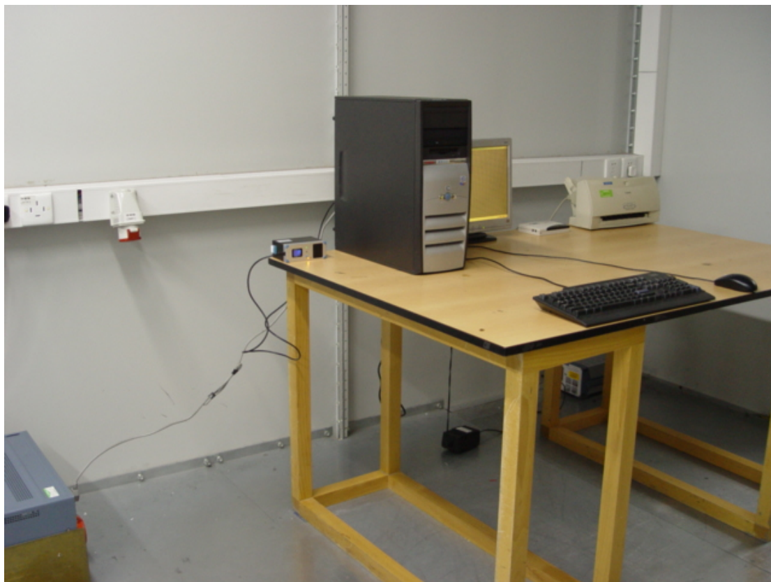
Photo 1 Conducted Emission test
