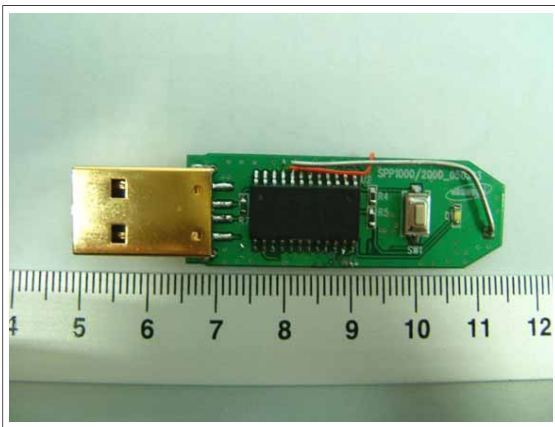
View 9 (SPP1500R)
