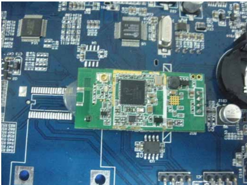
Photo 6 General Appearance of the EUT ( inside )
