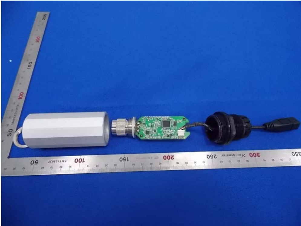
(1) EUT Photo(AWUHN2408)
