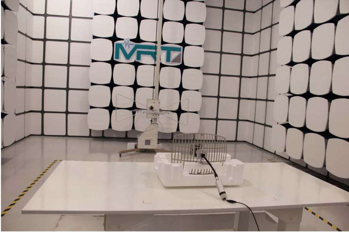
Description: Radiated Emission Test Setup for Below 1GHz (Antenna AG-24015)
