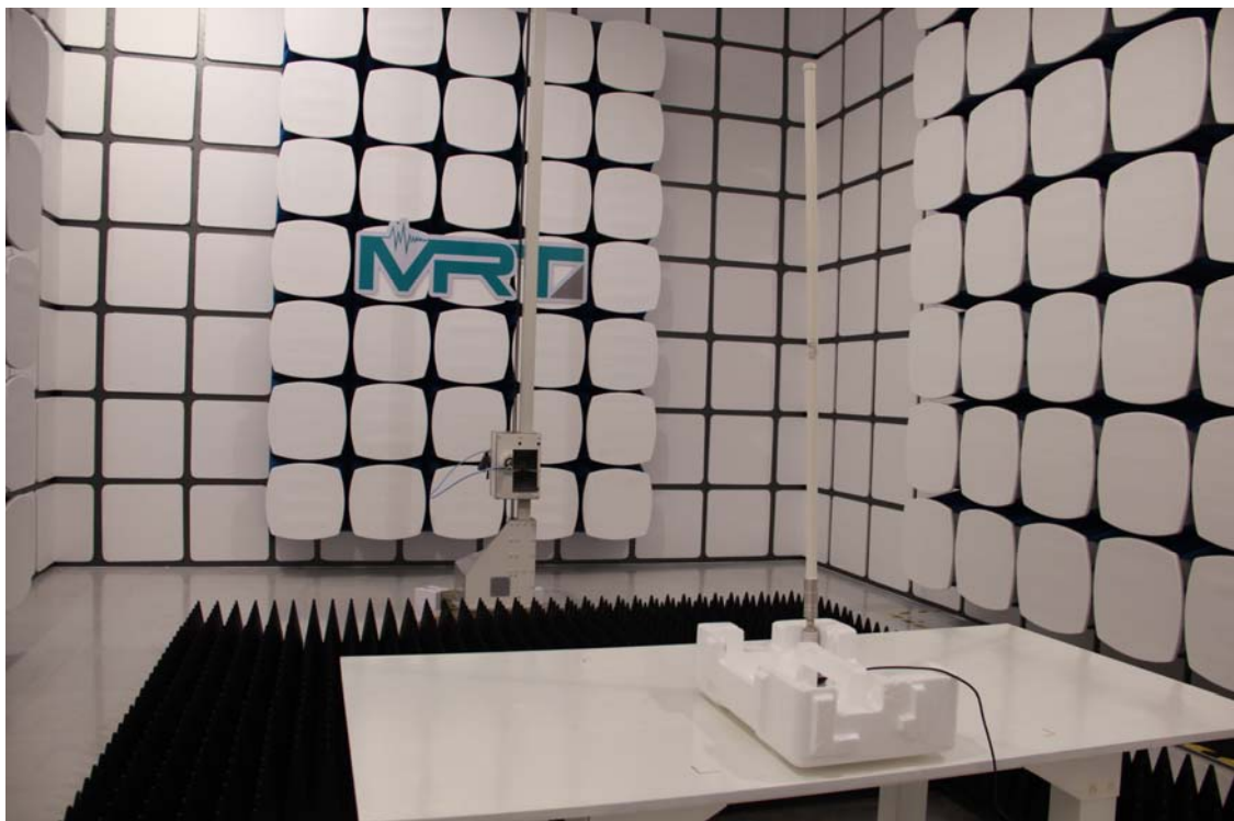
Description: Radiated Emission Test Setup for 1~18GHz (Antenna AO-24015)
