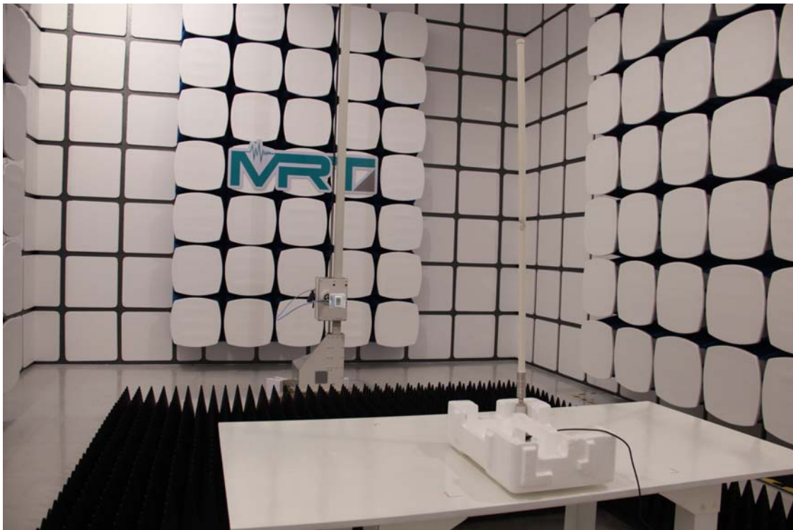
Description: Radiated Emission Test Setup for Above 18GHz (Antenna AO-24015)
