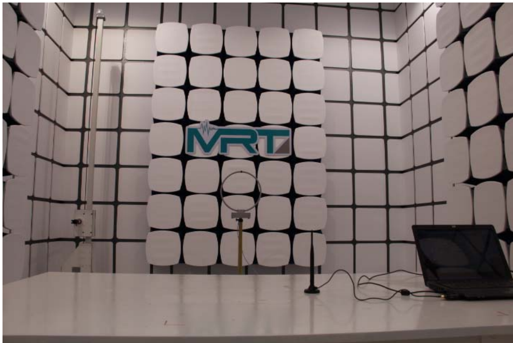
Description: Radiated Emission Test Setup for Below 30MHz(With Antenna A-2409D)
