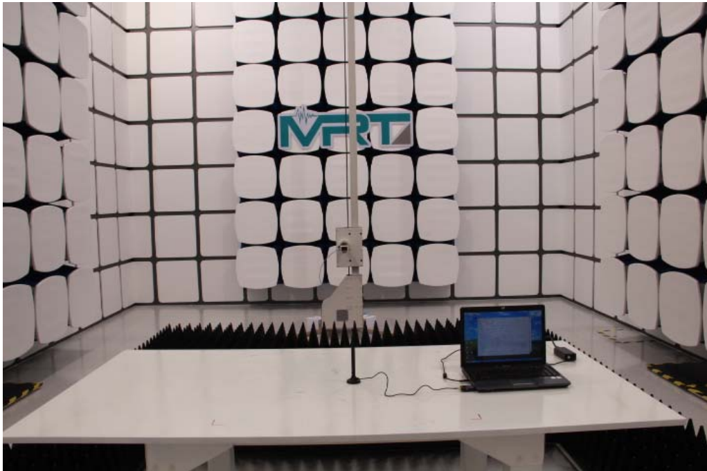
Description: Radiated Emission Test Setup for Above 18GHz(With Antenna A-2409D)
