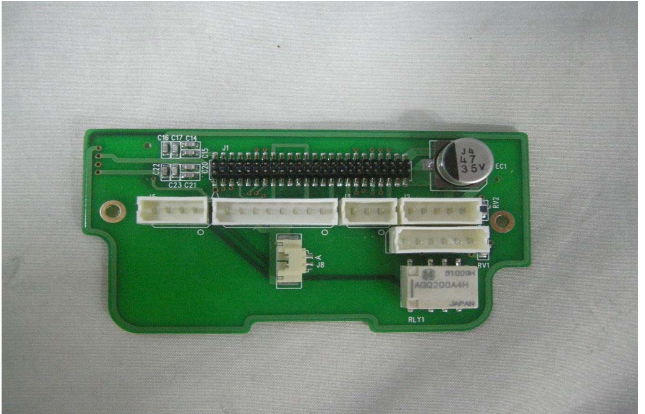
IO & antenna Board 1
